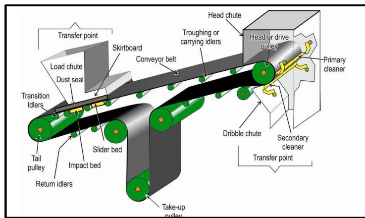
Gambar 4. Belt Conveyor
