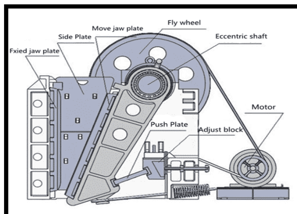
Gambar 2. Jaw Crusher
