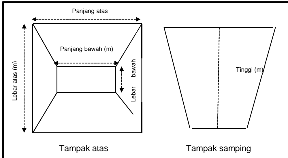
Gambar 1. Hopper Geometry
