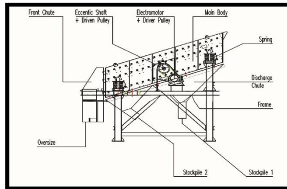
Gambar 3. Vibrating Screen
